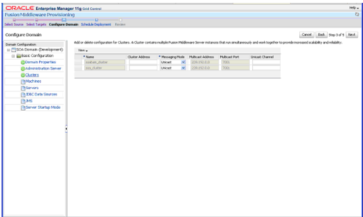
Figure 13–8 Clusters Page
