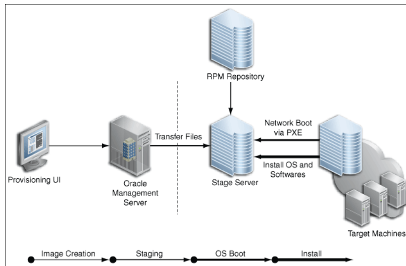
Figure 2–1 User Flow for Creating Deployable Images for Hardware Servers
