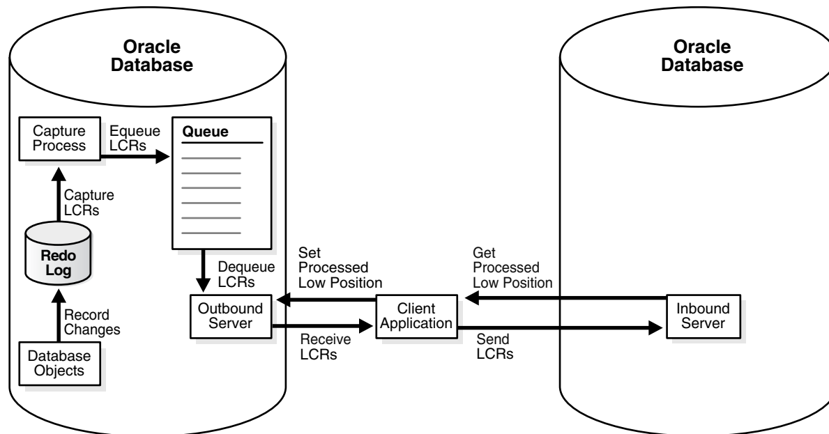
Figure 3–1 Sample XStream Configuration
