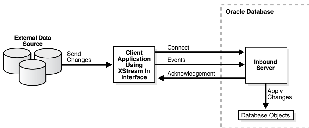
Figure 1–3 XStream In Inbound Server
