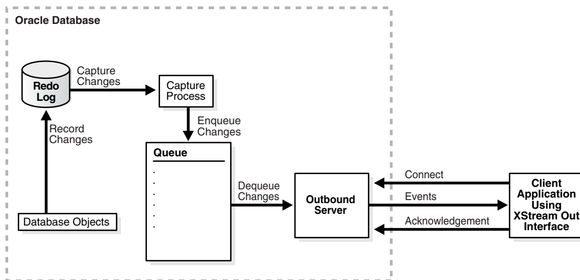
Figure 1–2 XStream Out Outbound Server
