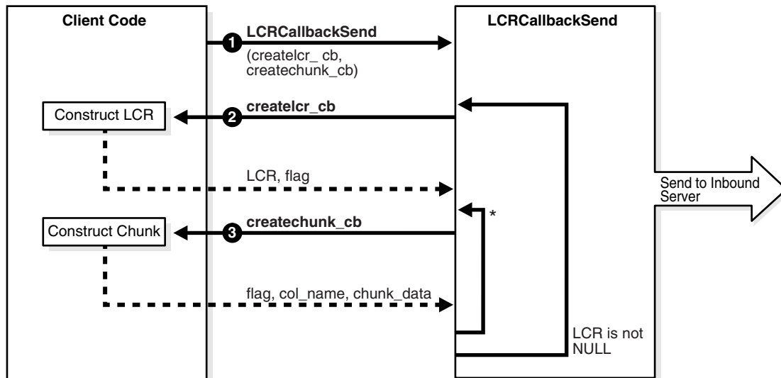
Figure 10–1 Execution Flow of the OCIStreamInLCRCallbackSend() Function
