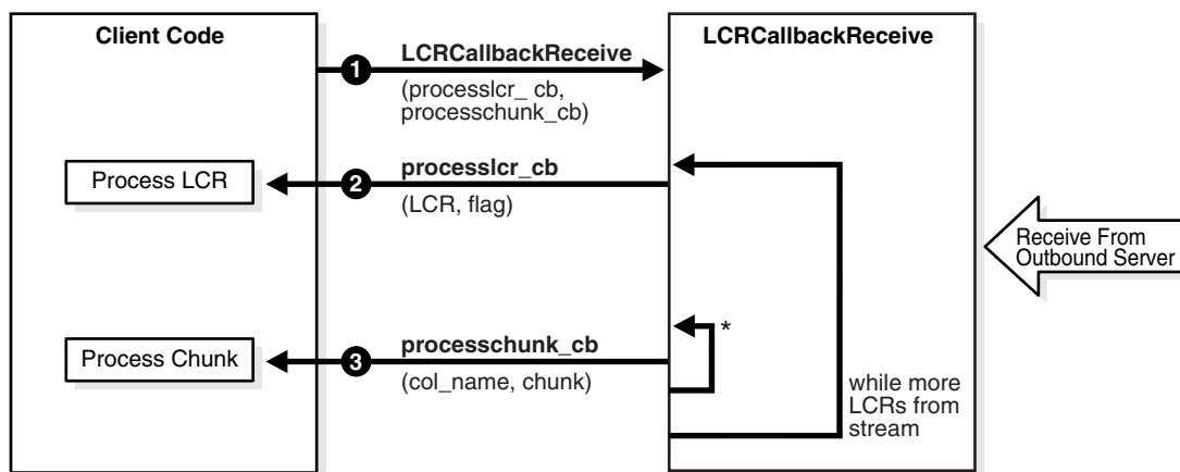
Figure 10-2 Execution Flow of the OCIXStreamOutLCRCallbackReceive() Function
